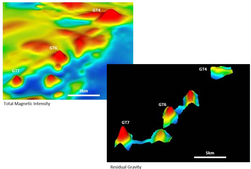
[Figure 1] Gulf Project: Gibson's Tank 3D oblique topographic view of the total magnetic intensity image (top left) and the residual gravity images from Red Metal's surveying (bottom right).
