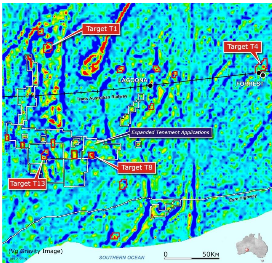
[Figure 8] Red Metal Nullarbor Project: Vertical gradient gravity colour image showing Red Metal's granted tenements (white/red) and new applications (white/black) and initial targets for proof of concept drill tests.
