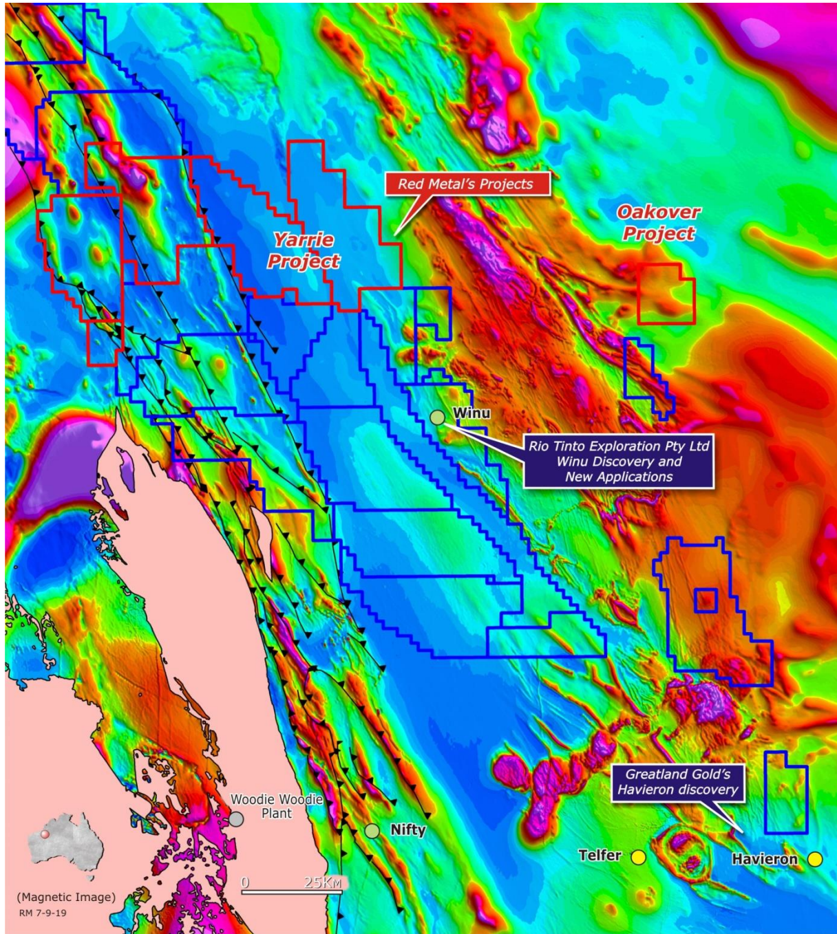
[Figure 9] Paterson Province Yarrrie and Oakover Projects: Magnetic imagery with Nifty Mine, Telfer Mine, Haverion prospect, Winu prospects and Red Metal's Yarrrie and new Oakover tenement applications (red line) and Rio Tinto Exploration Pty Limited's new applications (blue line). Note the exposed basement terrain of older Archaean rocks (buff coloured polygon).
