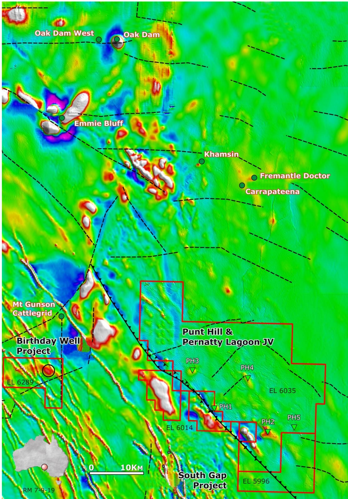
[Figure 12] Birthday Well Project, Punt Hill and Pernatty Lagoon Joint Venture Project: Total magnetic image showing the location of the Birthday Well airborne electromagnetic conductor (black circle) in relation to the Punt Hill and Pernatty Lagoon tenements and the Carrapateena, Khamsin and Oak Dam copper and gold deposits.
