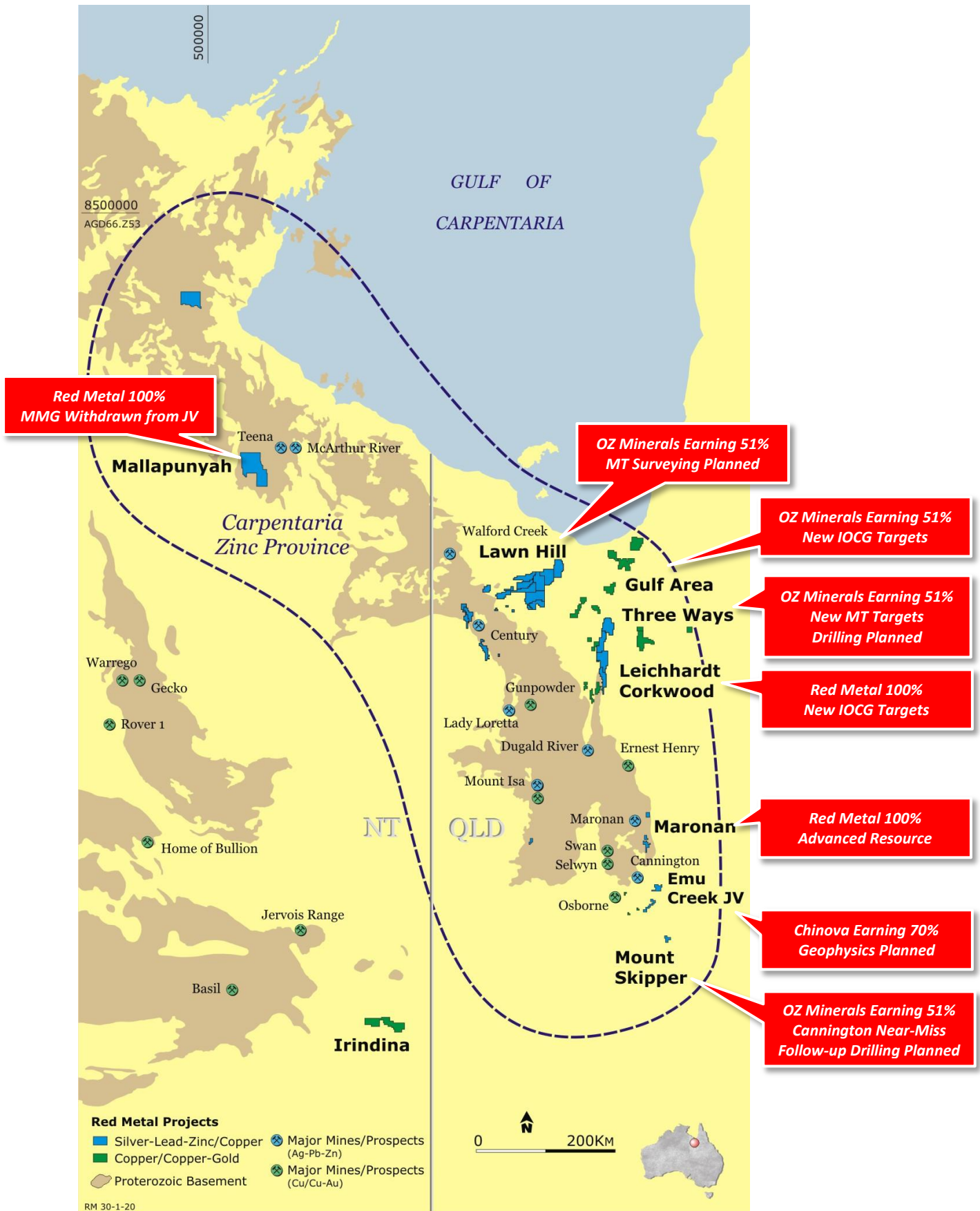
[Figure 1] Northwest Queensland and Northern Territory: Major deposits and Red Metal tenement locations.
