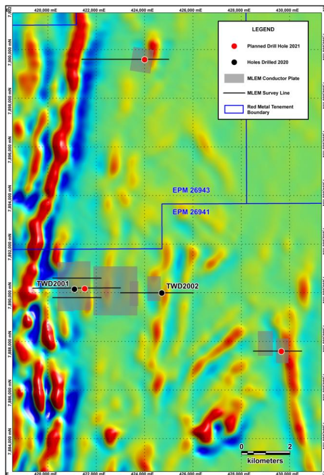
[Figure 1] Three Ways Project: Vertical gradient magnetic image showing moving loop ground electromagnetic lines, near-miss drill holes TWD2001 and TWD2002 and the current planned drill holes (red).
